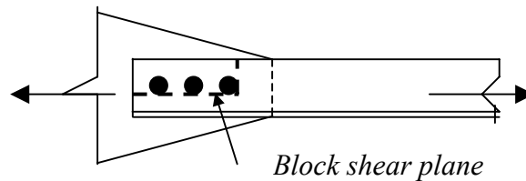
Fig. 9 Block Shear Failure
