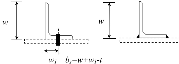
Fig 8 Angles with End Connection
