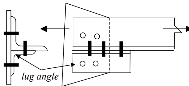
Fig. 10 Tension Member with Lug
