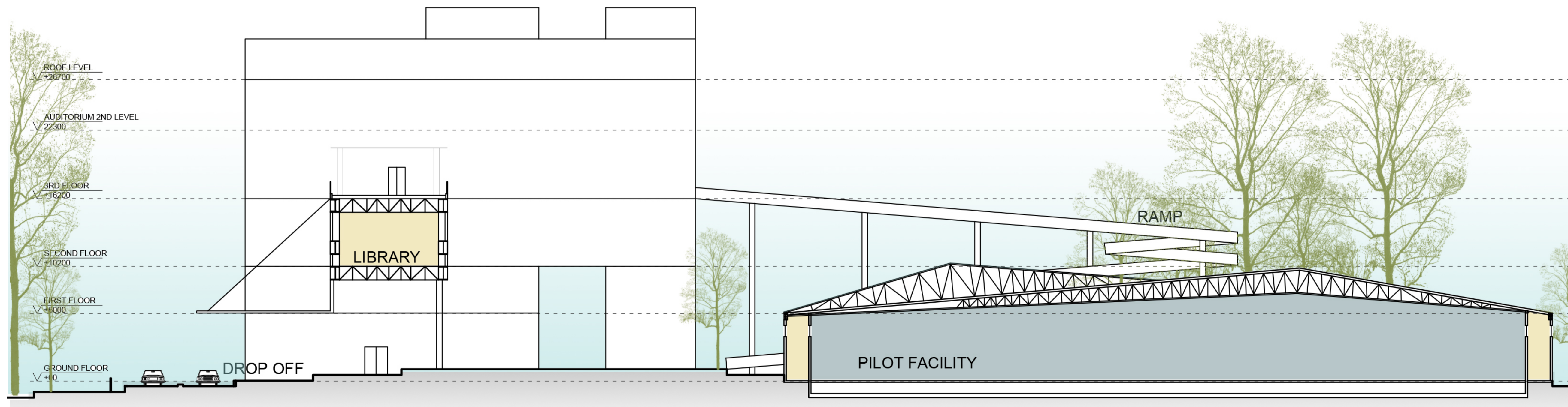
SECTION B-B' Scale - 1:200
