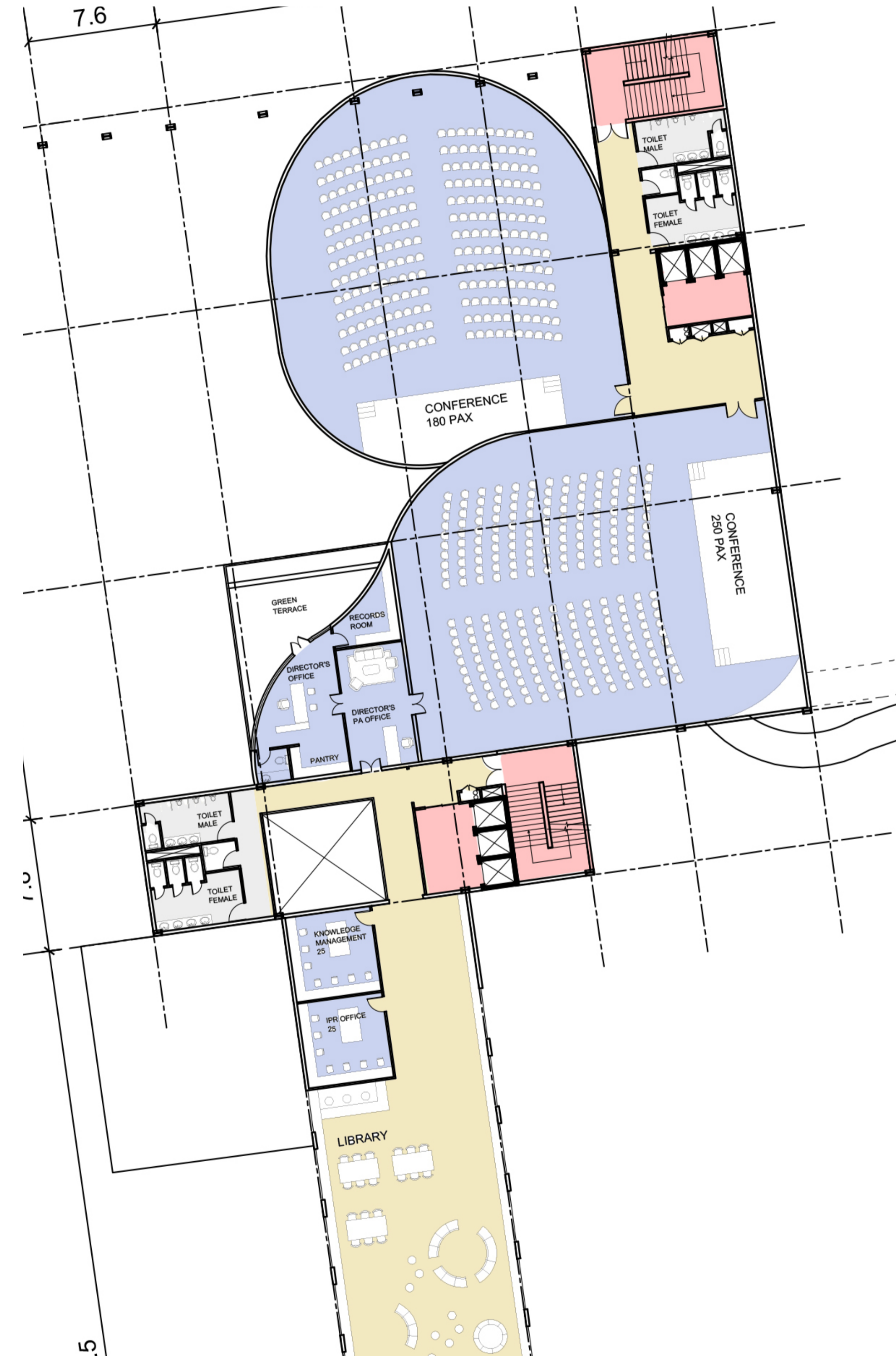
SECOND FLOOR LVL +10200 Scale - 1:200
