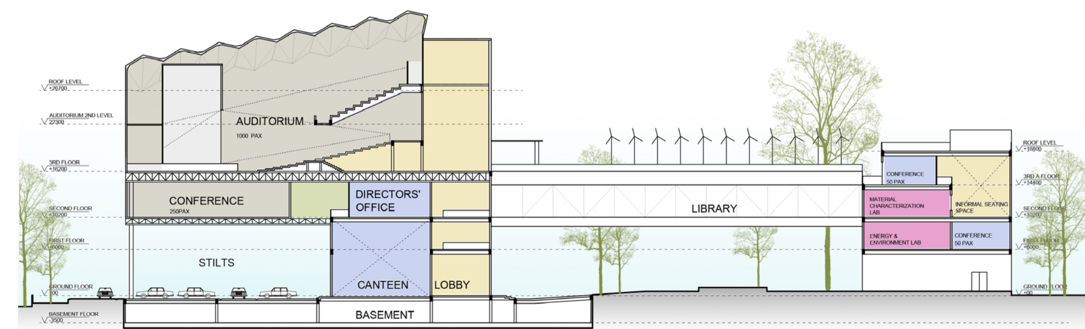
SECTION A-A' Scale - 1:500
