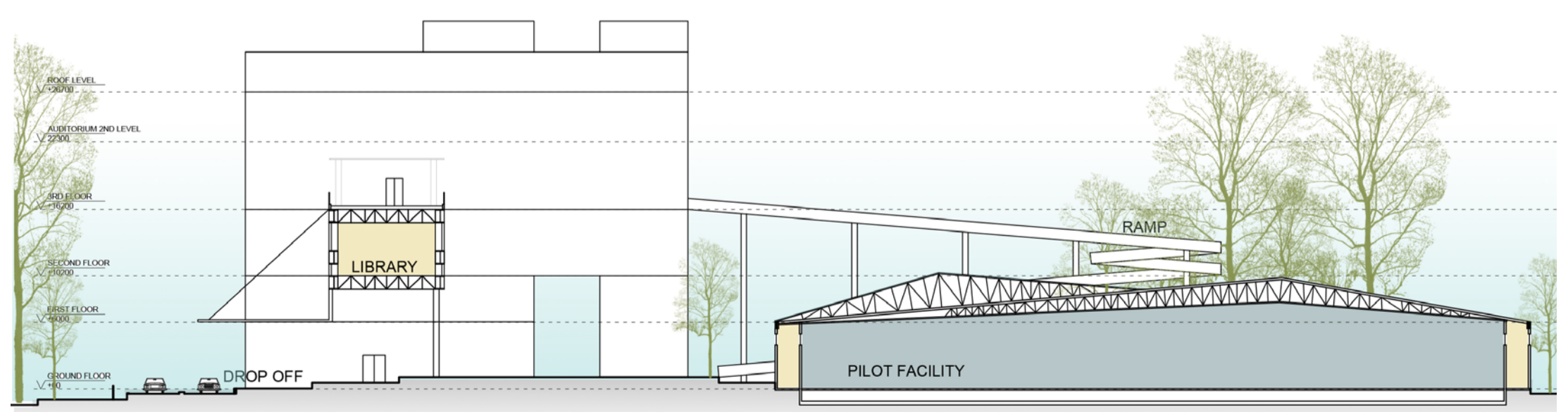
SECTION B-B' Scale - 1:500
