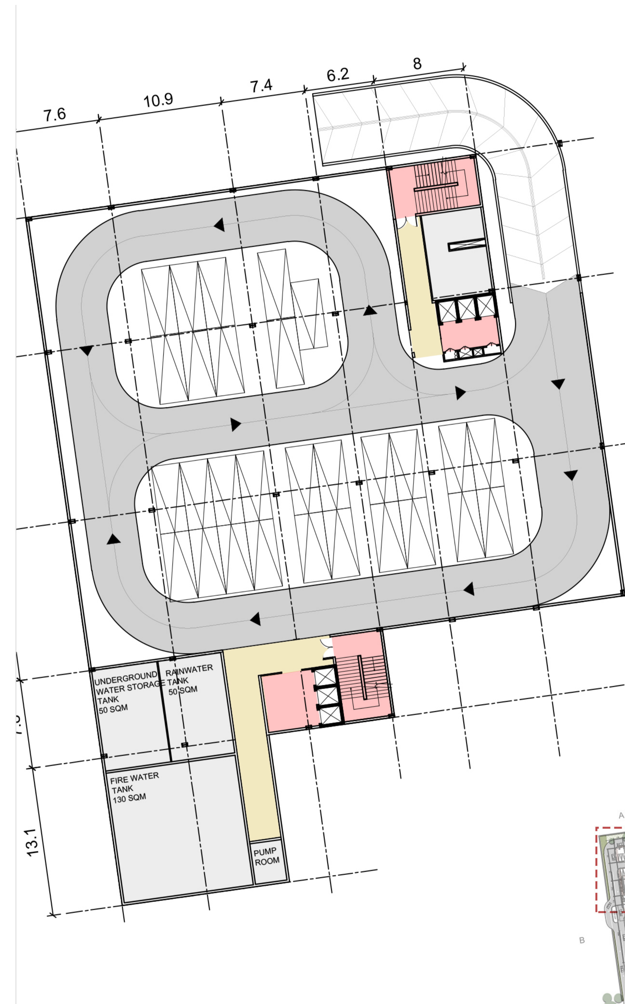
BASEMENT LEVEL LVL -3500 Scale - 1:200
