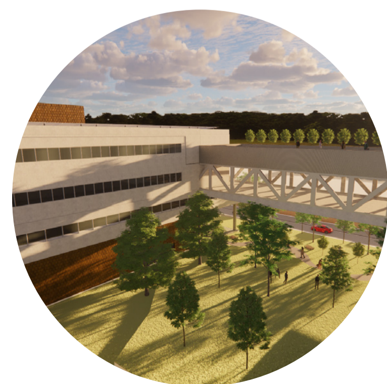
STRIP WINDOWS WITH LIGHT SHELVES AT 2100 MM HEIGHT FOR LABS
